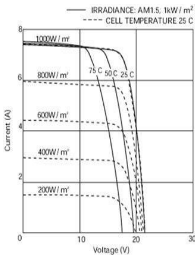
Figure 10. Temperature Effect on I-V Curve.
