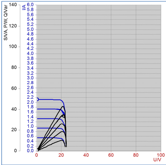
Figure 5. Getting the Fill Factor From the I-V Sweep was taken “EPH 2 Advanced photovoltaics trainer”.
