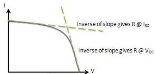
Figure 7. Obtaining Resistances from the I-V Curve.
