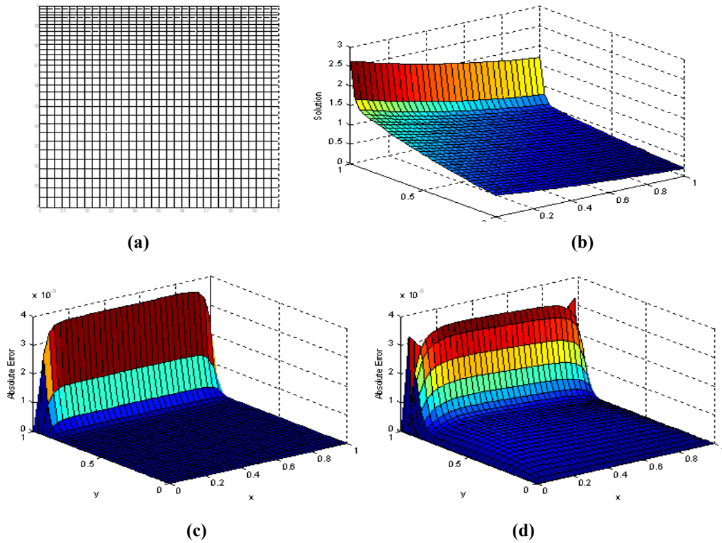
Figure 2. Results of Problem 1 for \epsilon = 0.01 on grid 32^3 in plane z = 0.5625 (a) Non-uniform grid ( \lambda_x = \lambda_z = 0 , \lambda_y = 0.55 ); (b) exact solution; (c) absolute error on uniform grid; (d) absolute error on non-uniform grid.
