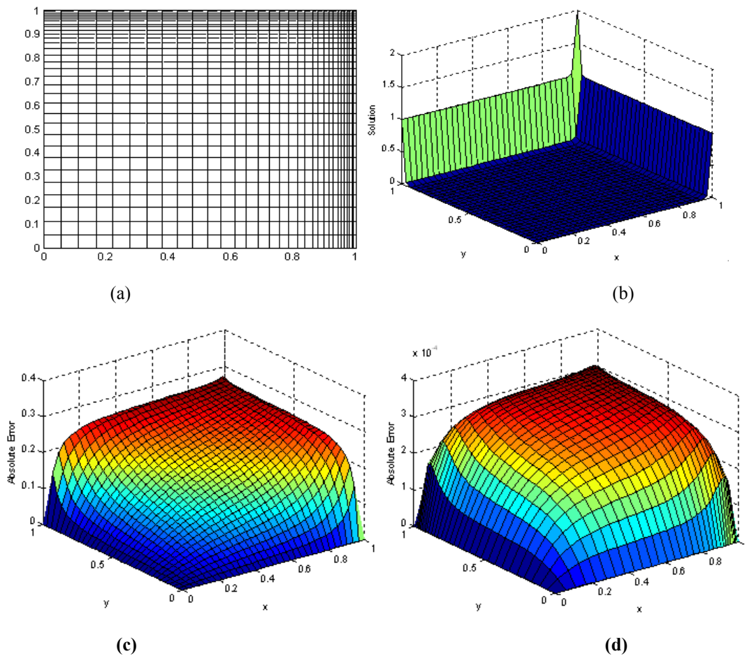
Figure 3. Results of Problem 2 at plane z = 0.8125 (uniform grid) and plane z = 0.8123 (non-uniform grid) for \epsilon = 0.01 ( \lambda_x = \lambda_y = \lambda_z = 0.8, 32^3 ), (a) Non-uniform grid, (b) exact solution, absolute error on (c) uniform grid, and (d) non-uniform grid.
