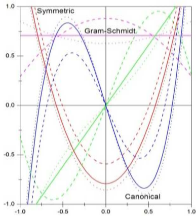
Figure 1. Unified view of Legendre and Löwdin-Legendre Polynomials
