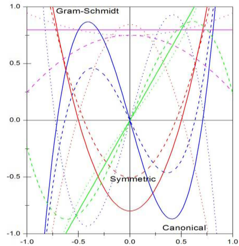
Figure 5. Unified view of Chebyshev II and Löwdin-Chebyshev II Polynomials
