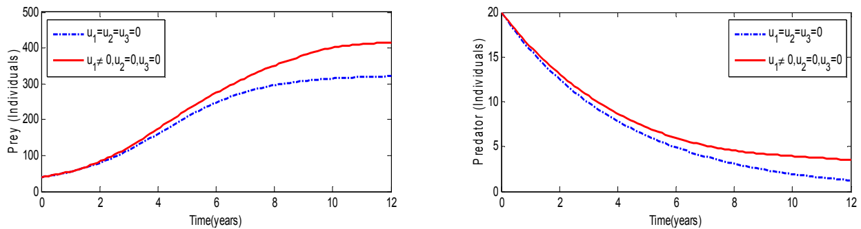
Fig. 2a. Simulations of a threatened prey-predator model showing the effect of optimal application of anti-poaching patrols.
