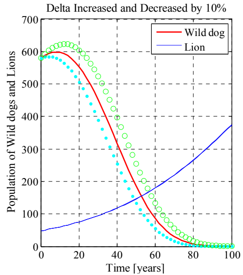
Figure 2. Changes in the solution of the system (1) and (2) on increasing and decreasing the parameter value by 10 percent.
