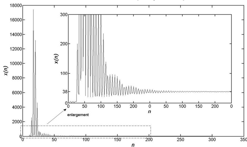
Figure 2. The solution of equation (4), when initial values x_{-3} = x_{-6} = x_{-9} = 0.05 , x_0 = x_{-1} = x_{-2} = x_{-4} = x_{-5} = x_{-7} = x_{-8} = 10 .
