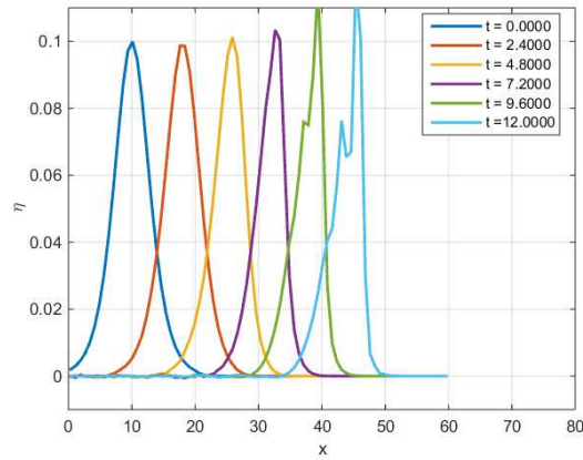
Figure 3. Solution plots of interaction of soliton-to-bottom with different bottom geometries: bottom geometry 1, 2, and 3 (from top to bottom).
