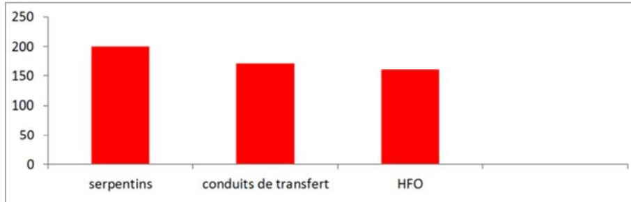
Figure 4. Temperature Histograms DEUTZ.
