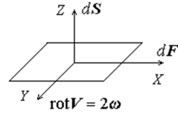
Figure 1. The directions of vectors in the formula (33).
