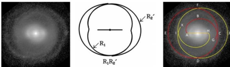
Figure 15. Left: NGC 1079, original image; middle: Spiral arm profile depicted by Buta; right: Simulation by ROTASE model.
