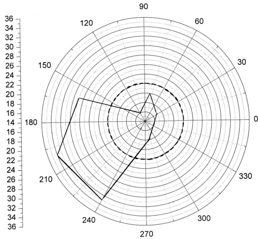
Fig 2. Distribution of observed angles \zeta (solid line). Dashed line shows the expected uniform distribution.
