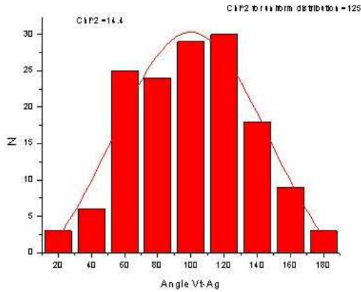
Fig 6. Alternative presentation of the distribution of angles \epsilon .
