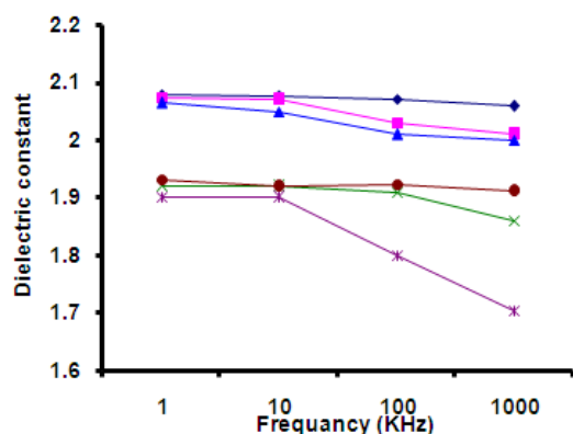
Fig (5) The dielectric constant (ε') vs. frequency at temperature 35°C S 0 , S 1 , S 2 , S 3 , S 4 and S 5 greases
