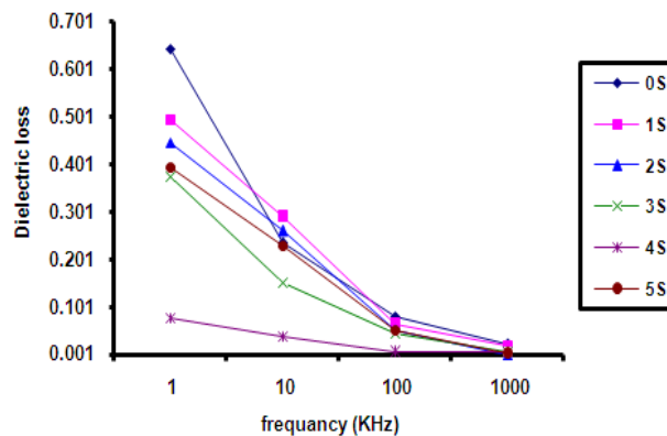
Fig (6) The dielectric loss (ε'') vs. frequency at temperature 35°C S 0 , S 1 , S 2 , S 3 , S 4 and S 5 greases
