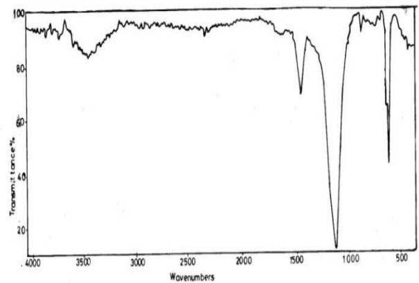
Fig. (5) IR spectrum of silicon dioxide
