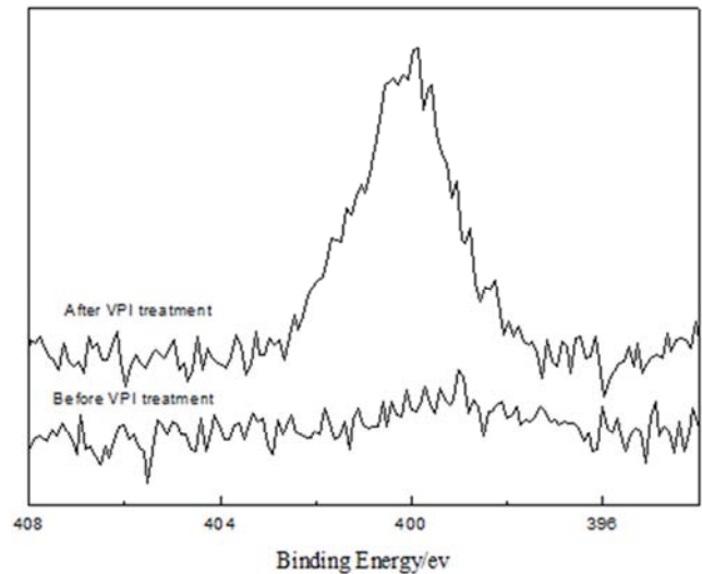
Fig. 9. XPS spectra of nitrogen element on coin surface.
