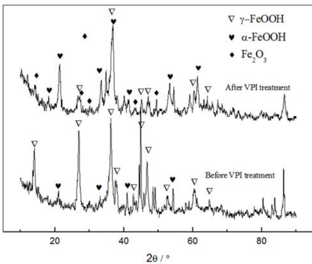
Fig. 4. XRD of surface rust of cast iron before and after inhibition treatment.
