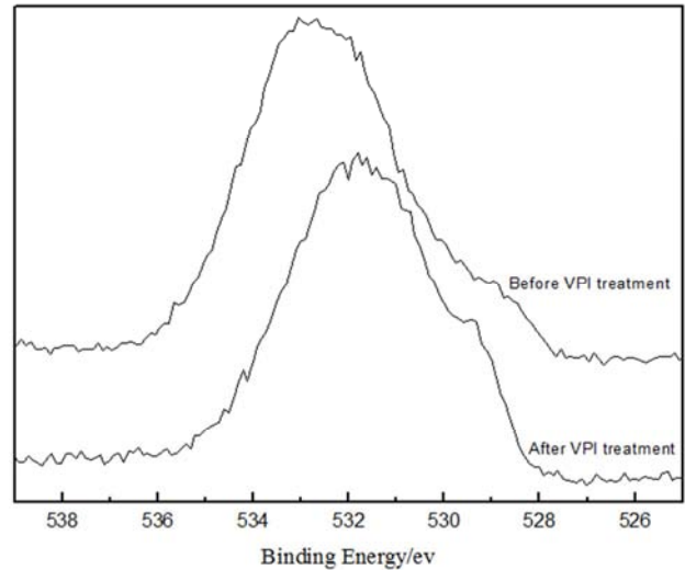
Fig. 8. XPS spectra of oxygen element on coin surface.
