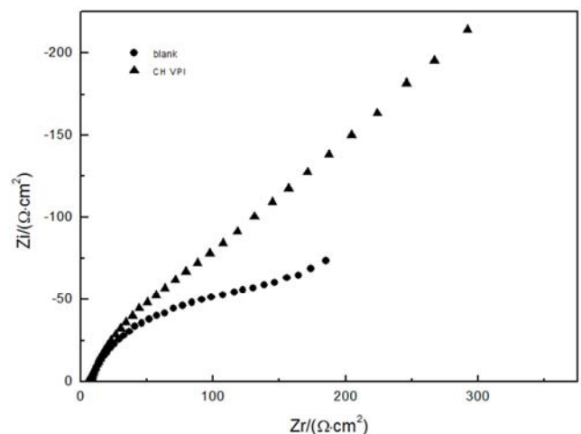
Fig. 2. Electrochemical impedance spectroscopy in solution with or without CH VPI.
