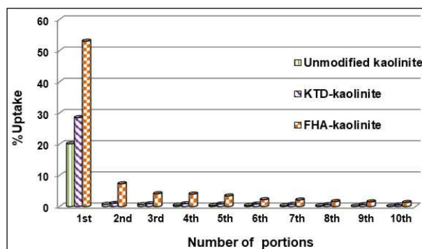
Figure 11. % Uptake of Cd (II) by unmodified and both modified kaolinite clay using column technique.
