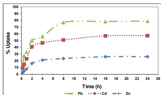
Figure 5. Effect of contact time on the amount of adsorption of Pb (II), Cd (II) and Zn (II) by KTD-kaolinite clay.
