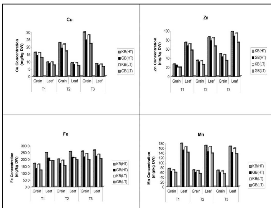
Figure 1. The content builds up of metallic cations in the dry weight of fronds and grain of two beans (KB: Red Bean GB: Green Bean HT: Sandy clay LT: Sandy loam).
