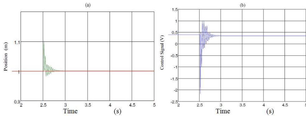
Figure 4. System motion curve response based on fuzzy controller (Shoulder Axis).
