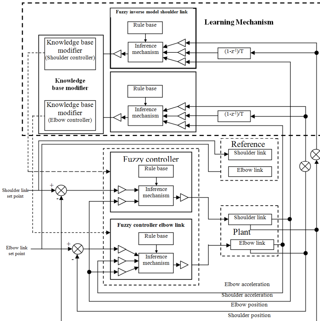
Figure 1. FLMRC for the two link robot.
