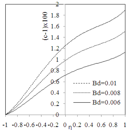
Fig 7. The graphs of the concentration profile c(\eta) against the width of the channel taking \psi = \pi/9, M=0.5, P_r E_c=0.01, t_d=0.01, R_E=10, R_m=2 for the various values of baro-diffusion number.
