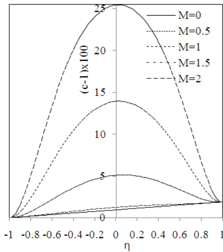
Fig 6. The graphs of the concentration profile c(\eta) against the width of the channel taking \psi = \pi/9, R_E=10, R_m=2, Pr E_c=0.01, B_d=0.01, t_d=0.01 for the various values of the Hartmann number.
