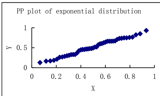
Fig. 4. Exponential distribution of PP plot.
