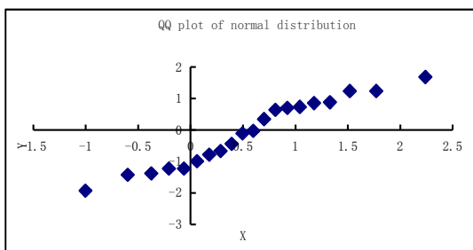
Fig. 5. Normal distribution of QQ plo.
