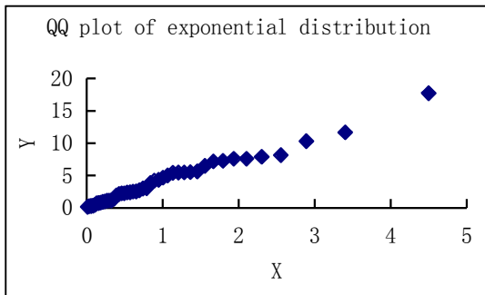
Fig. 3. Exponential distribution of QQ plot.
