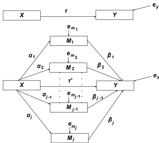
Figure 2. A multiple mediator model
