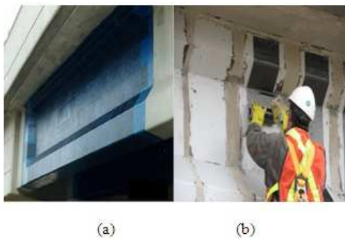
Figure 1. Shear strengthening of Reinforced concrete using CFRP laminate
