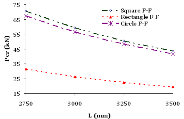
Figure 3. Variations of the buckling loads of FEM for steel columns with three different equivalent cross sections versus length under F-F boundary conditions (E = 2×10 5 MPa , A = 3600 mm 2 )
