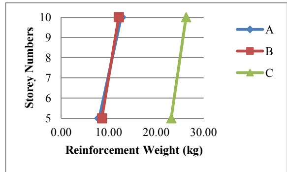
Figure 9. Required reinforcement for beams vs. storey number.
