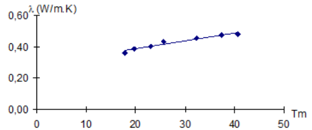
Figure 13. Variation of conductivity as a function of the average temperature: earth and straw (N'Djamena).
