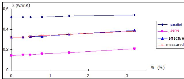
Figure 15. Calculated and measured thermal conductivity variations: earthhand straw (N'Djamena).
