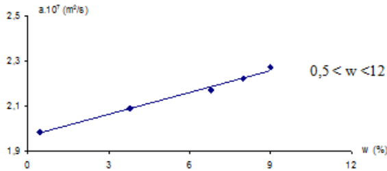
Figure 6. Variation of the diffusivity as a function of water content: Earth only (N'Djamena).
