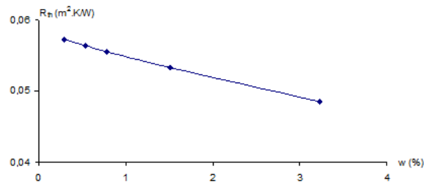
Figure 11. Variation of thermal resistance as a function of water content: earth and straw (N'Djamena).
