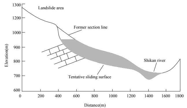
Figure 3. Schematic diagram of Wenjiaba landslide profile.
