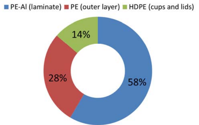
Figure 2. PE-Al composition obtained in hydropulping process as dry mass % (excluding residual paper which varies from 1-15%).
