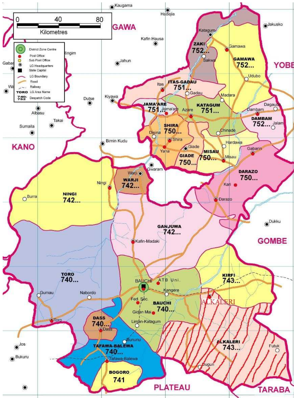
Figure 1. Location map of Alkaleri Kaolin Deposit.
