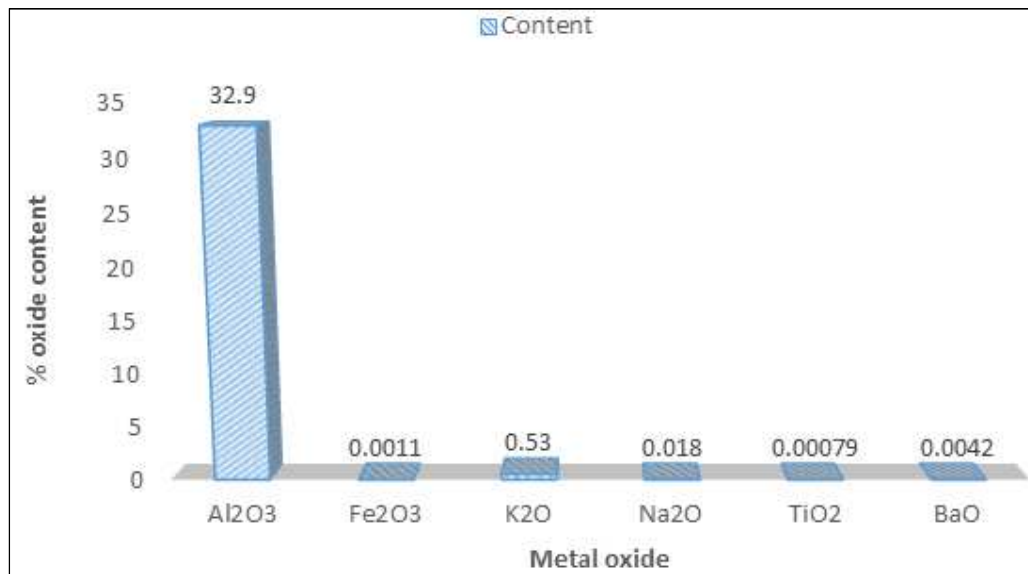
Figure 2. Percentage oxide content of Alkaleri Kaolin.
