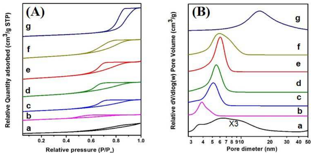
Figure 3. (A) \text{N}_2 adsorption-desorption isotherms and (B) corresponding pore size distributions of various alumina samples. (a) Com- \text{Al}_2\text{O}_3 , (b) \text{Al}_2\text{O}_3 -0, (c) \text{Al}_2\text{O}_3 -0.125, (d) \text{Al}_2\text{O}_3 -0.25, (e) \text{Al}_2\text{O}_3 -0.375, (f) \text{Al}_2\text{O}_3 -0.5, (g) \text{Al}_2\text{O}_3 -0.75.
