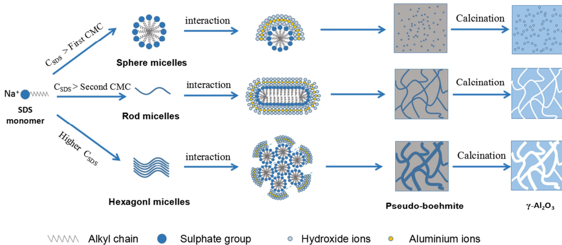
Figure 5. Transformation of SDS micelles at different concentrations and the proposed mechanism of SDS addition effect on the texture of resultant \gamma\text{-Al}_2\text{O}_3 .
