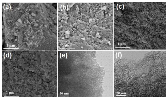
Figure 4. SEM images of alumina samples of (a) Com- \text{Al}_2\text{O}_3 , (b) \text{Al}_2\text{O}_3 -0, (c) \text{Al}_2\text{O}_3 -0.25, (d) \text{Al}_2\text{O}_3 -0.375, and the corresponding TEM images of (e) \text{Al}_2\text{O}_3 -0, (f) \text{Al}_2\text{O}_3 -0.375.
