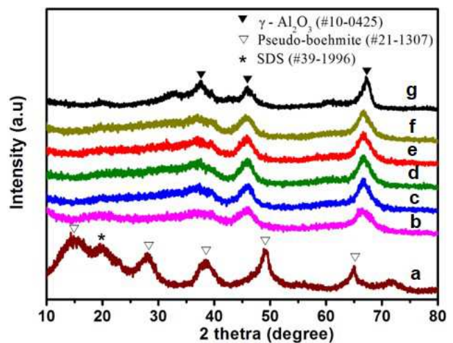
Figure 2. XRD patterns of different materials involved. (a) pseudo boehmite-0.375, (b) \text{Al}_2\text{O}_3\text{-0} , (c) \text{Al}_2\text{O}_3\text{-0.125} , (d) \text{Al}_2\text{O}_3\text{-0.25} , (e) \text{Al}_2\text{O}_3\text{-0.375} , (f) \text{Al}_2\text{O}_3\text{-0.5} , (g) \text{Com-Al}_2\text{O}_3 .
