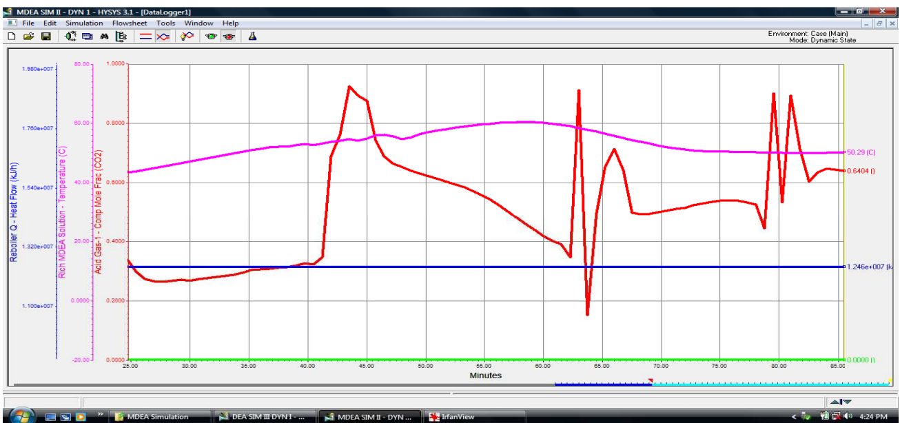
Figure 2. Strip chart showing real time variables for MDEA Simulation Case.
