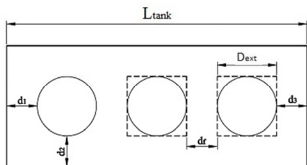
Figure 1. Layout of the HV winding to the transformer tank.
