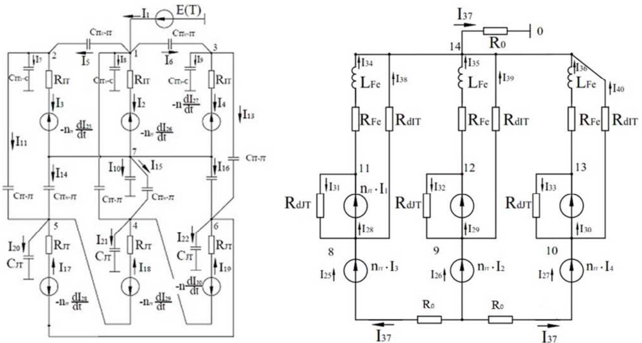
Figure 2. Coupled circuits model.
