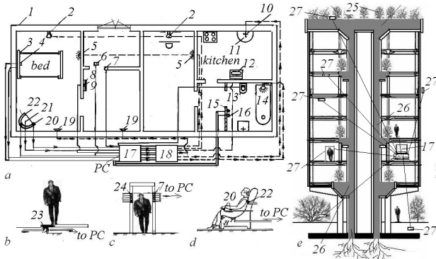
Figure 3. Plan of intellectual home with the indication of the locations of detectors (sensors) and effectors (executive mechanisms) (a); details (b-d); soil-filled building (e): 1 - external wall; 2 - spray for supply of aerosols; 3 - resistive-strain sensors on bed; 4 - sensor (receiver) of exhaled air; 5 - lighter with color filters; 6 - sensors of weight of body in floor; 7 - photo resistors in a jamb of door; 8 - mirror; 9 - transmitting color TV camera; 10 - supply of medicinal additives in potable water; 11 - wash-bowl; 12 - display with conclusion of the data on a recommended diet and a healthy way of life; 13 - the sensors in «clever» toilet; 14 - tube for introduction of medicinal additives in water in douche and in bath; 15 - thermo vision camera; 16 - equipment for control by method Kirlian - effect; 17 - system of executive mechanisms; 18 - microprocessor; 19 - loudspeaker; 20 - sensors of blood pressure and heartbeat; 21 - resistive-strain sensors in sitting of armchair; 22 - microphone; 23 - sensors of shuffling in floor; 24 - sources of light; 25 - green roof; 26 - soil in vertical canals; 27 - soil on floors
