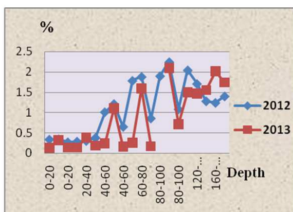
Fig. 5. Total Amount (%) of Dry Residue (Tsnori, plot without drainage) for 2012 and 2013.
