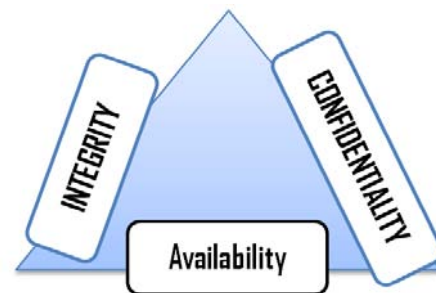
Figure 5. CIA Triad.
