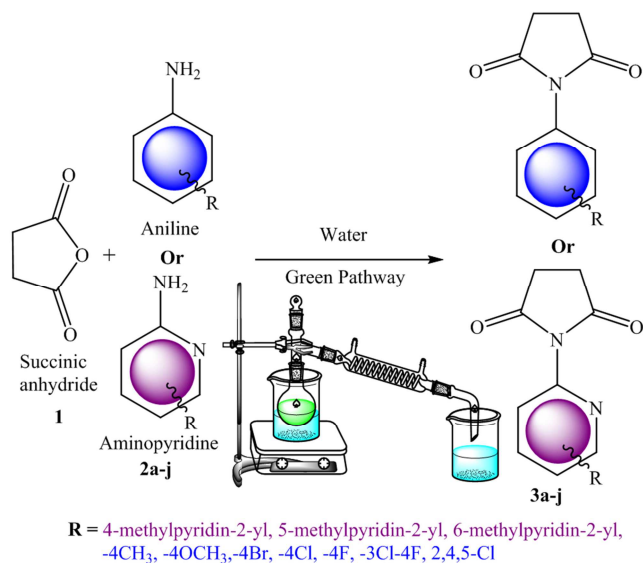
Figure 1. Synthesis of N-phenyl or N-methylpyridin-2-yl succinimides (3a-j).
