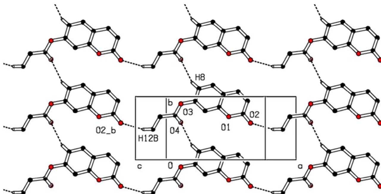
Figure 5. Part of the crystal packing of the title compound showing the formation of an infinite R_s^4(30) motifs in the ab plane. Dashed lines indicate hydrogen bonds. H atoms not involved in hydrogen bonding have been omitted for clarity.
