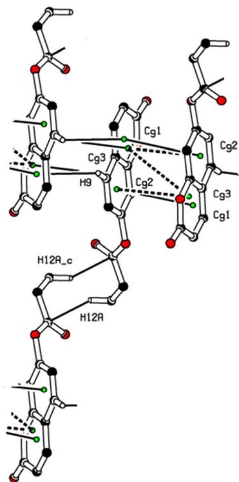
Figure 6. A view of the crystal packing, showing H...C contacts, C-H... \pi and \pi - \pi stacking interactions (dashed lines). The green dots are ring centroids. H atoms not involved in H...C or H... \pi interactions have been omitted for clarity.
