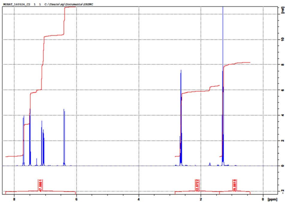
Figure 2. ^1\text{H} NMR Spectrum of (1) in \text{CDCl}_3 .
