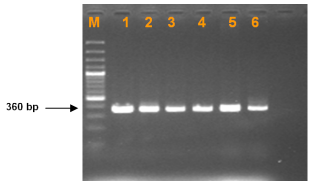
Figure 6. Agarose gel gel electrophoresis of PCR products obtained by amplifying nif-H gene from genomic DNA of bacterial isolates. M, marker 100bp DNA ladder, 1-6 were 6 strains among 73 strains.
