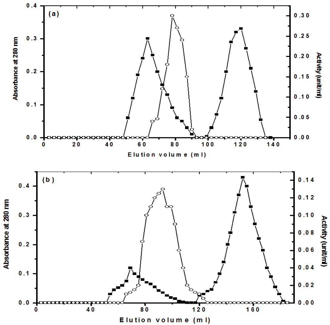
Fig. 2. Typical elution profiles for the chromatography of T. alexandrinum of dormant GST2 (a) and germinated GST3 (b) seeds on Sephadex G-100 column at a flow rate of 20 ml/h and 3 ml fractions volume. Absorbance at 280 nm (•), GST activity at 340 nm (◦).
