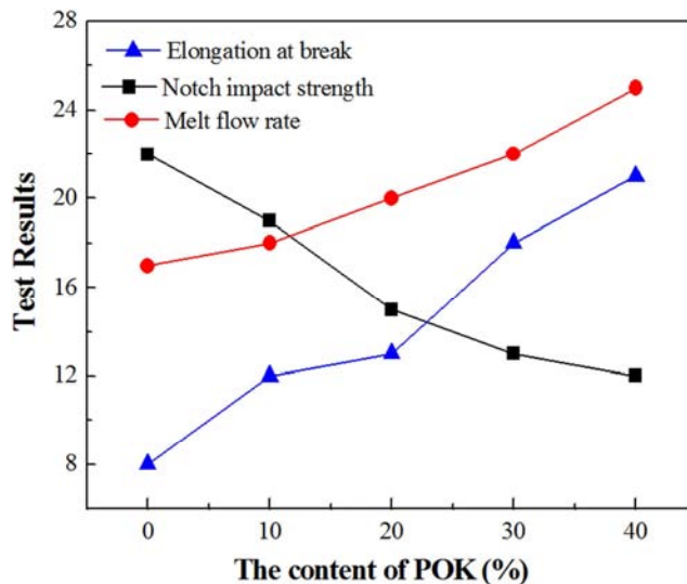
Figure 5. Mechanical properties of alloy materials with different POK resin contents.
