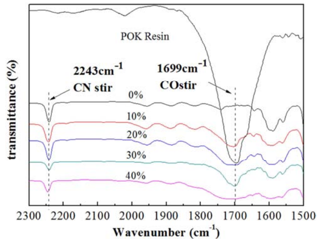
Figure 1. FT-IR spectral of flame retardant ABS polyketo alloy.
