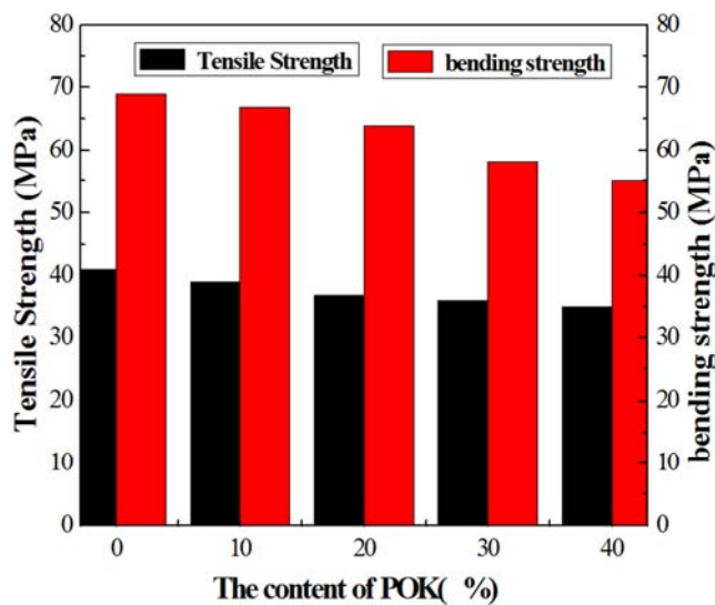
Figure 4. Tensile Strength and bending strength properties of alloy materials with different POK resin contents.
