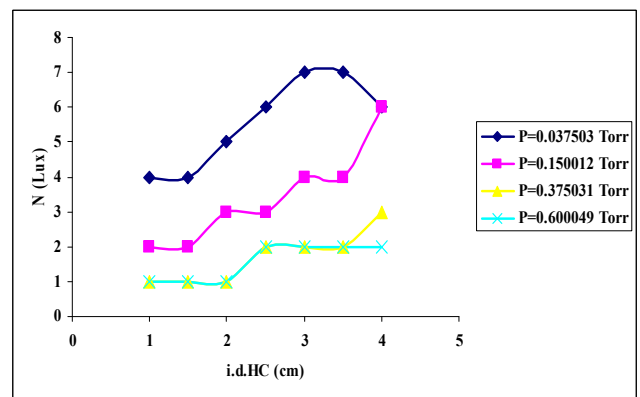
Figure 8. Luminous intensity as a function of depth of hollow cathode at different pressures.
