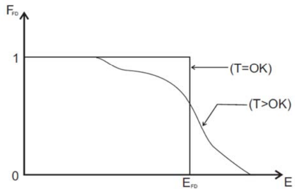
Figure 2. Plots of F_{FD} Versus Energy E for T=0K and for T>0K for a metal.
