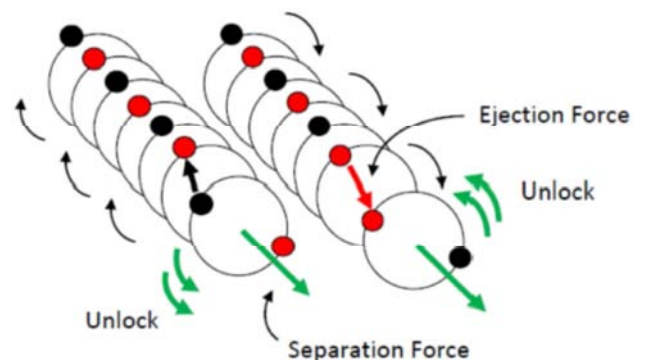
Figure 1. Photon Formed in a two stage process by releasing Wu's Pair from its Parent Substance.
