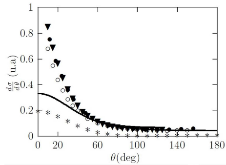
Figure 2. Differential cross section for 50 eV. Star symbols are the present first Born with exchange. Full circle curve is from Shyn [29], open circle are from D. F. Register et al. [1] and full triangle are from M. J. Brunger et al. [8]. Solid line is from relativist calculations of A. Jablonski et al. [28].
