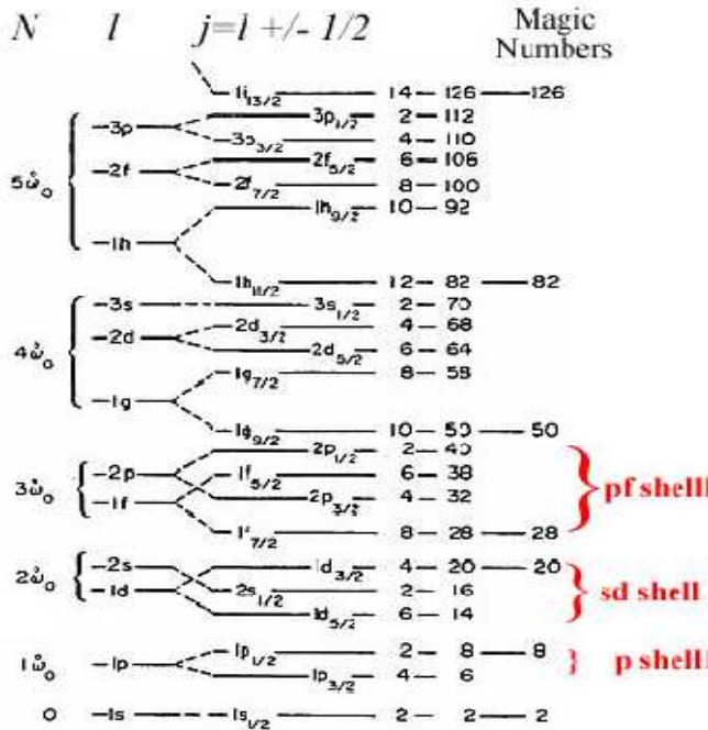
Figure 1. p, sd and pf shell model spaces.
