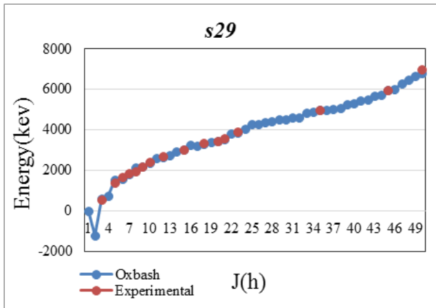
Figure 2. Comparison Calculated data with Experimental data for 29 S.
