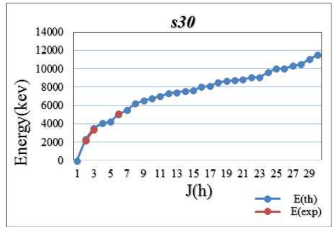
Figure 3. Comparison Calculated data with Experimental data for 30 S.
