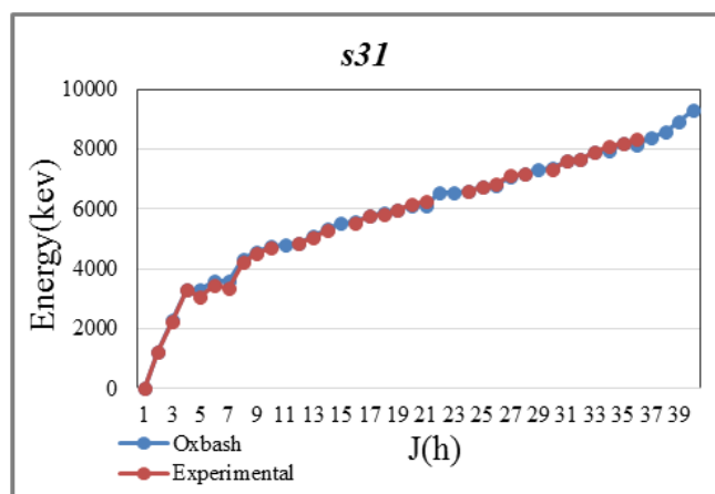
Figure 4. Comparison Calculated data with Experimental data for ^{31}\text{S} .
