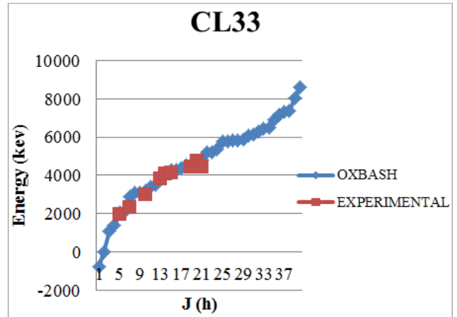
Figure 3. Comparison Calculated data with Experimental data for 33 Cl.
