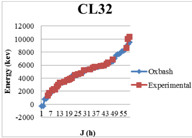
Figure 2. Comparison Calculated data with Experimental data for 32 Cl.
