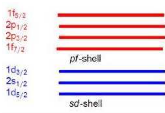
Figure 1. PF and SD model spaces
