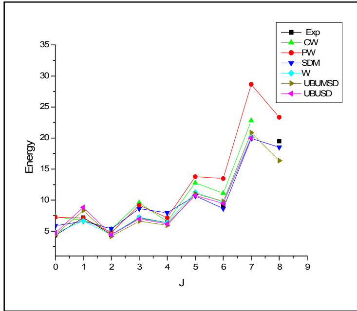
Figure2. Resulted curves for energy levels of 36 Ar by applying 6 interacting suitable potentials in SD space model 1d_{3/2} 1d_{5/2} 2s_{1/2} and comparing with experimental data.
