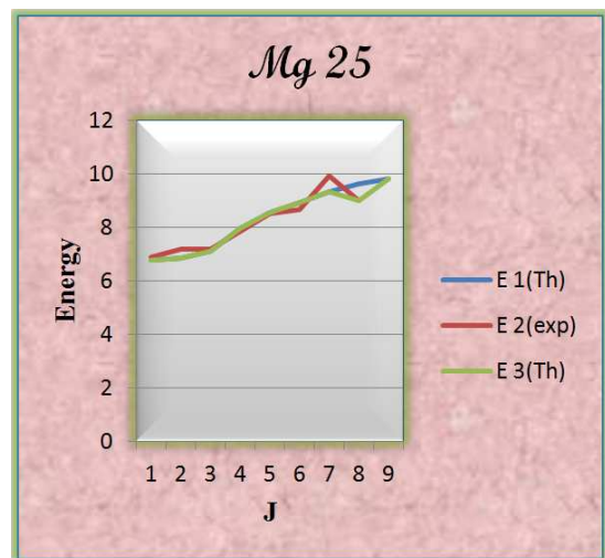
Figure 3. Comparison Calculated data with Experimental data for 25 Mg.
