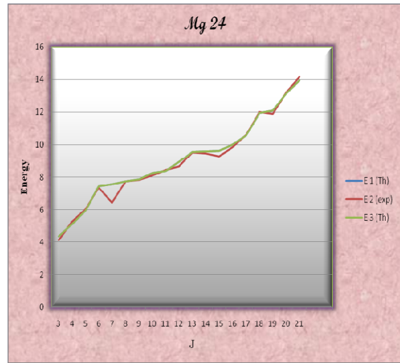
Figure 2. Comparison Calculated data with Experimental data for 24 Mg.
