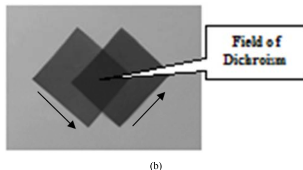
Figure 4. PVA-films containing the dye A in parallel (a) and perpendicular (b) directions of stretching.
