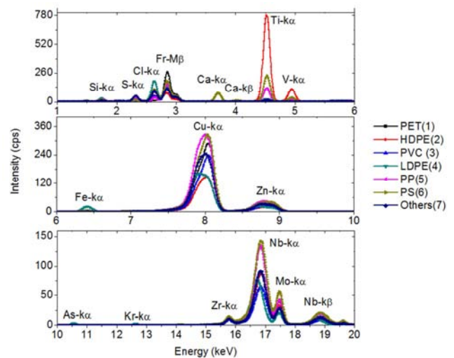
Figure 2. Intensity versus energy for various plastics of PET, HDPE, PVC, LDPE, PP, PS and Others calculated over the energy range from 1 to 20 KeV using XRF with RX9, Mo, Cu and Al targets.
