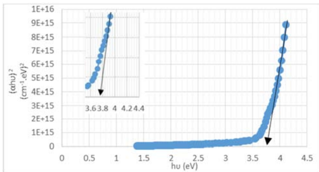
Figure 10. The variation of (ahv)^2 versus hv for Mg:SnO 2 (9wt%) film.
