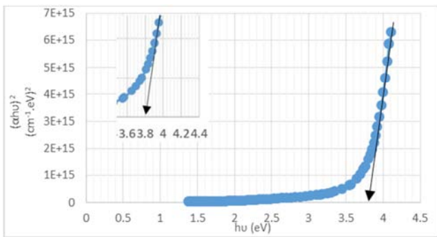
Figure 9. The variation of (ahv)^2 versus hv for Mg:SnO 2 (7wt%) film.
