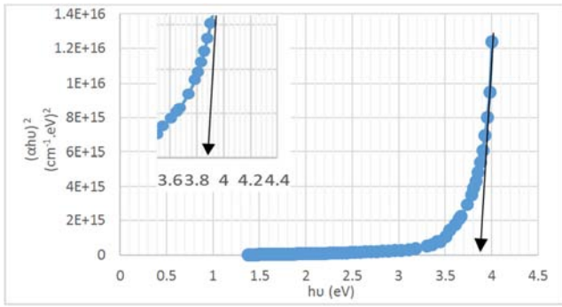
Figure 8. The variation of (ahv)^2 versus hv for Mg:SnO 2 (5wt%) film.
