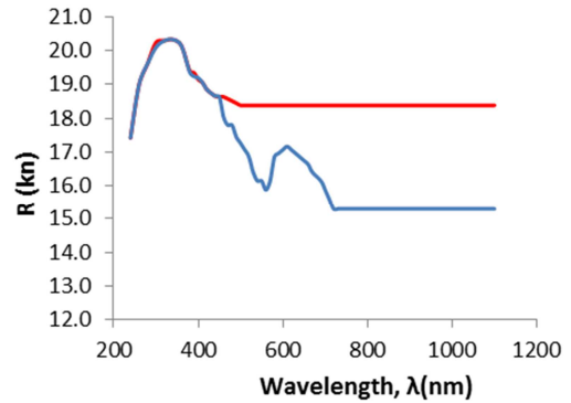
Figure 3. Spectral Reflectance of Thin Films of CuSbS 2 for 33G (red) and 33H (blue).
