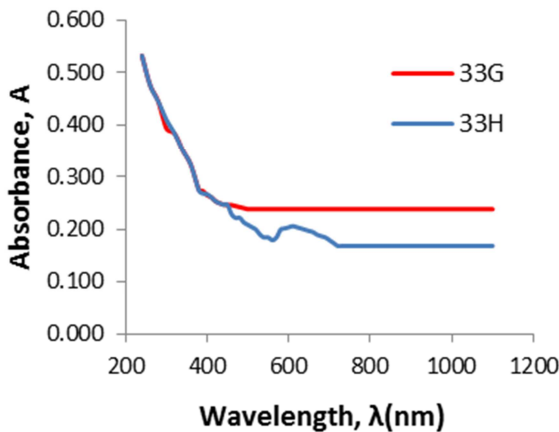
Figure 1. Spectral Absorbance of TF of CuSbS 2 .
