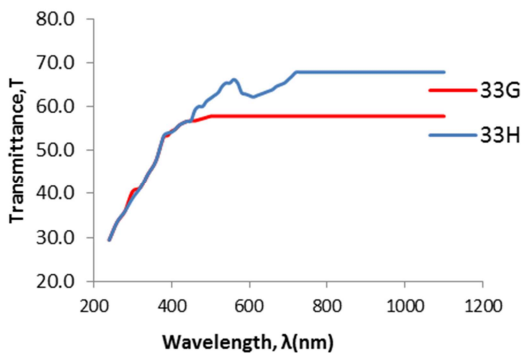
Figure 2. Spectral Transmittance of CuSbS 2 .
