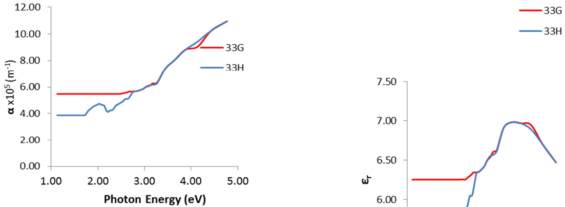
Figure 6. Absorption coefficient of Thin Films of CuSbS 2 .
