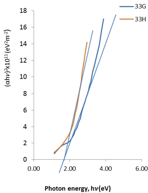
Figure 7. (\alpha h\nu)^2 versus photon energy for Thin Films of CuSbS 2 .
