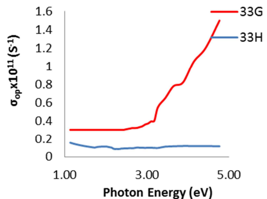
Figure 10. Optical conductivity of CuSbS 2 TFs.
