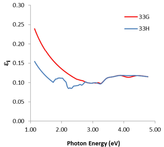
Figure 9. Imaginary dielectric constant versus photon energy CuSbS 2 .
