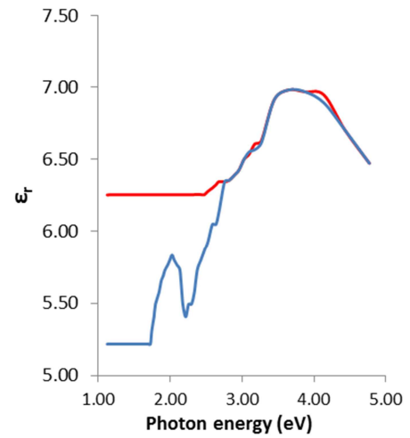
Figure 8. Real dielectric constant of TFs.
