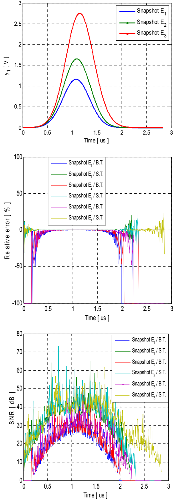
Figure 9. Snapshot of y_1 with the relative error and SNR using the time domain architecture.
