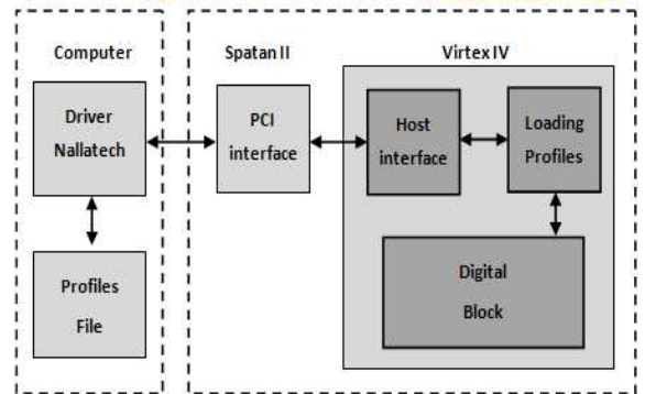
Figure 7. Connection between the computer and the XtremeDSP board.
